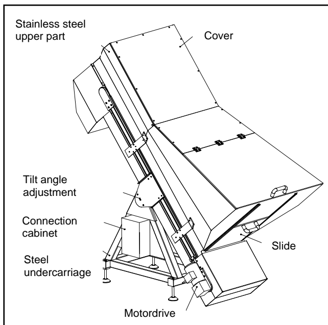
Figure 1 : main parts of the AAE bulkfeeders
